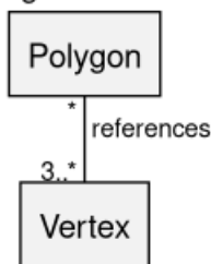
UML Class diagram: Association Example
